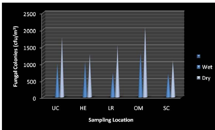
Figure 3: Seasonal Viable Counts of Fungi Isolated from Outdoor Ambient Air
