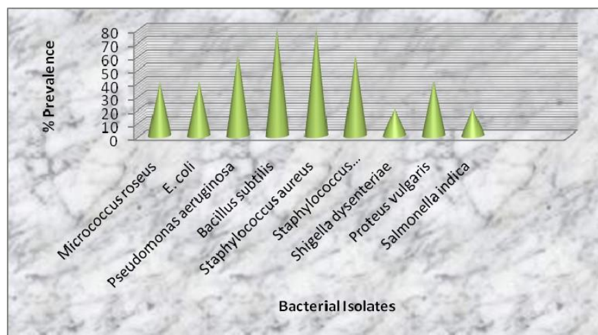
Figure 4: % Prevalence of Bacteria isolated from Outdoor Ambient Air during Wet Season
