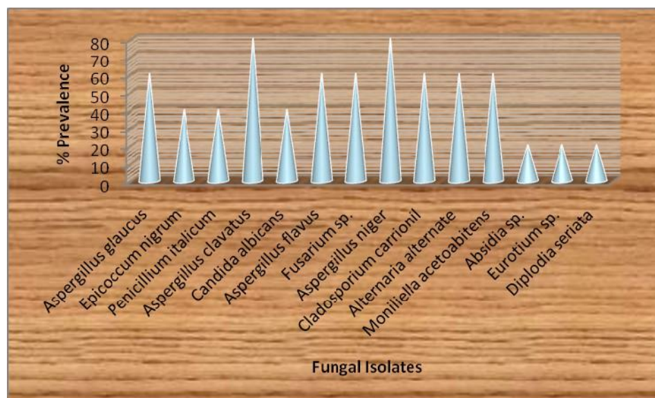
Figure 6: % Prevalence of Fungi isolated from Outdoor Ambient Air during Dry Season
