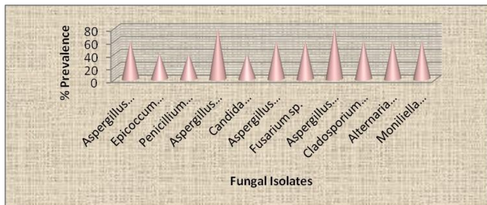
Figure 5: % Prevalence of Fungi isolated from Outdoor Ambient Air during Wet Season
