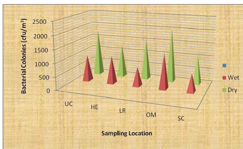
Figure 2: Seasonal Viable Counts of Bacteria Isolated from Outdoor Ambient Air
