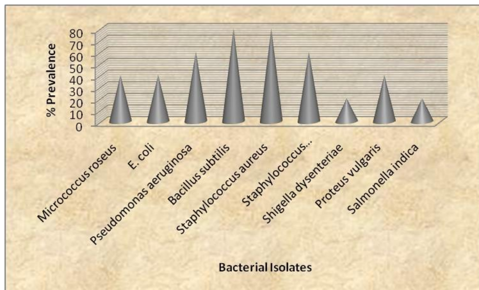
Figure 6: % Prevalence of Bacteria isolated from Outdoor Ambient Air during Dry Season
