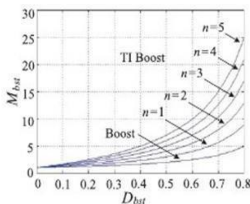
Fig. 6. Comparison of conversion ratio, M_{bst} , of the traditional boost and the TI boost converters.
