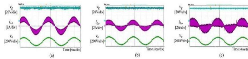
Fig 11. Experiment results of v_g , i_{Lo} , v_o under different output power ( V_g = 48 VDC): (a) 200W, (b) 100 W, (c) 50 W
