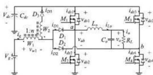
Fig 3.Topology presented in SSIB
