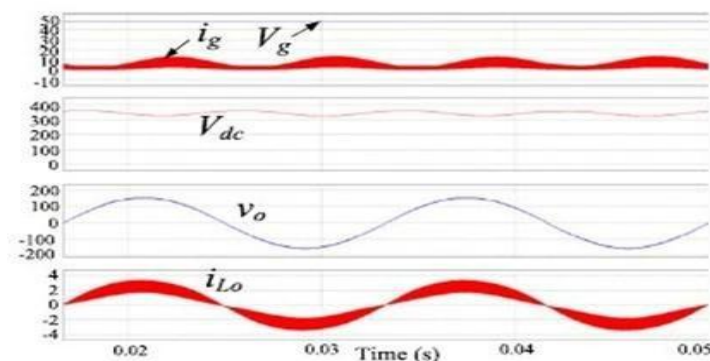
Fig 8. Simulated waveforms of the proposed SSBI on the line frequency
