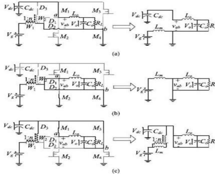
Fig 4.Topological states of the proposed SSBI
