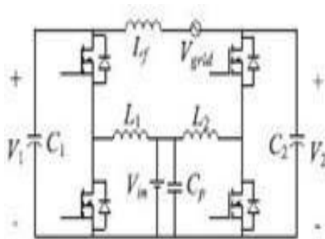
Fig 1(a).Topology presented in olden techniques
