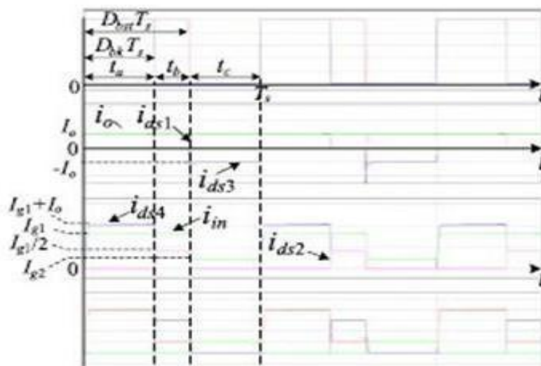
Fig. 7. Simulated waveforms of the proposed SSBI on the switching frequency scale during positive half-cycle.
