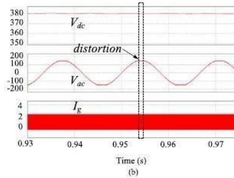
Fig. 10. Simulated waveforms of the SSBI's output voltage V_{ac} , dc-link voltage V_{dc} , and dc input source current I_g : (a) illustrating the undistorted output voltage V_{ac} , when SSBI is operated in deep DCM just above the minimum power level P_o > P_{o min} in and (b) illustrating the peak-shaving distortion of the output voltage V_{ac} for P_o < P_{o min} .
