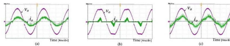
Fig. 12. Experimental results: SSBI's output voltage v_o and output current i_o under three different load conditions: (a) linear RL load, (b) nonlinear load case I: diode bridge with RC load, and (c) nonlinear load case II: resistor and saturable inductor load.
