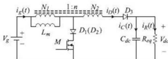
Fig. 9. Input voltage step-up scheme of the proposed SSBI (is identical to the TI boost converter).
