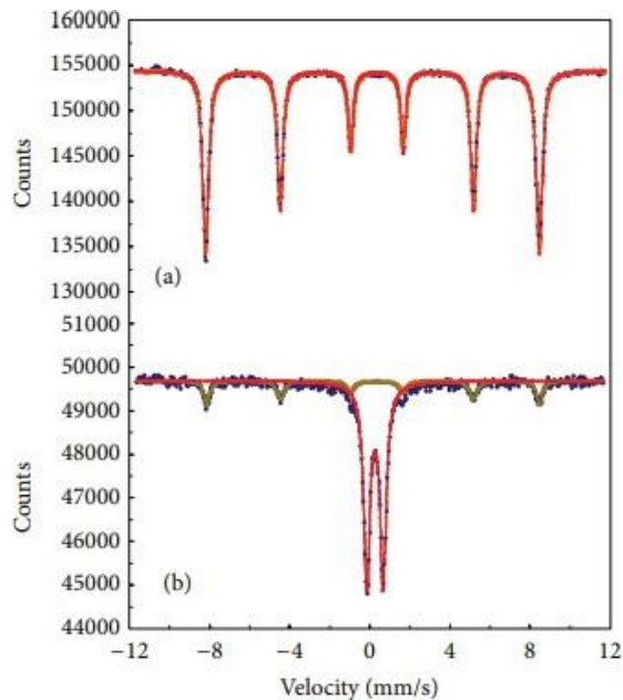
Figure 4: Mossbauer spectra at room temperature for \text{Fe}^{2+}\text{O}_3 and \text{CdFe}_2\text{O}_4 thermally treated at 500^\circ\text{C} for 3 h: (a) F500 and (b) CF500.
