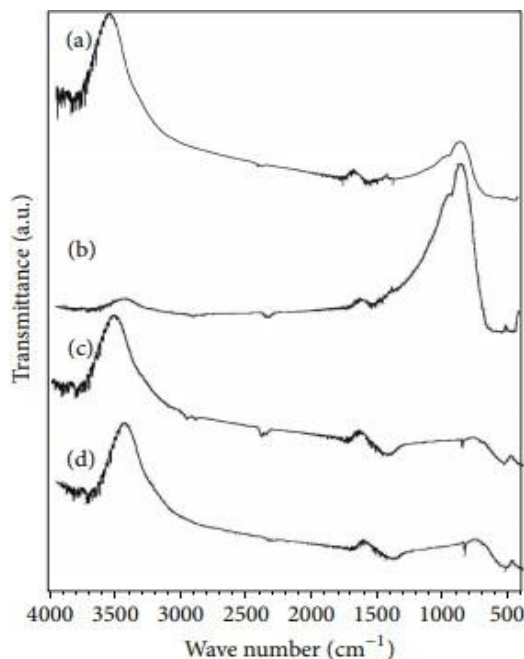
Figure 2: FTIR spectra of \text{Fe}_2\text{O}_3 and \text{CdFe}_2\text{O}_4 powders thermally treated at 500^\circ\text{C} and 600^\circ\text{C} for 3 h: (a) F500, (b) F600, (c) CF500, and (d) CF600.
