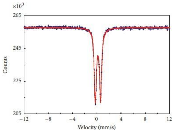
Figure 5: Mossbauer spectrum at room temperature for \text{CdFe}^{2+}\text{O}_4 thermally treated at 600^\circ\text{C} for 3 h: CF600
