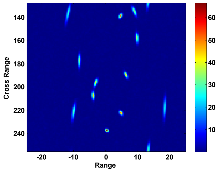
Fig.10. ISAR image using Gabor transform for F=15GHz
