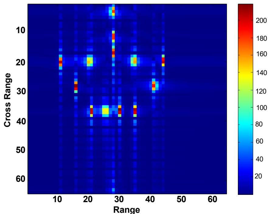
Fig.6. ISAR image using STFT for F=8\text{GHz}
