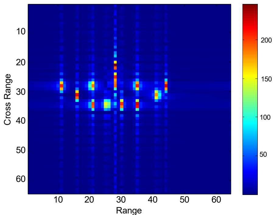
Fig.3. ISAR image using STFT for F=3GHz
