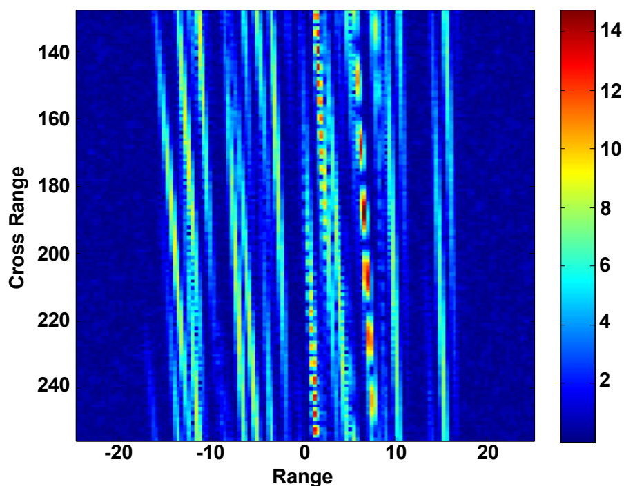
Fig.13 ISAR image using Gabor transform for F=40GHz
