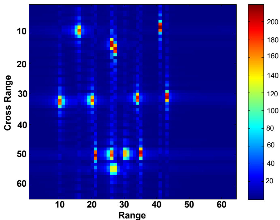
Fig.12. ISAR image using STFT for F=40\text{GHz}
