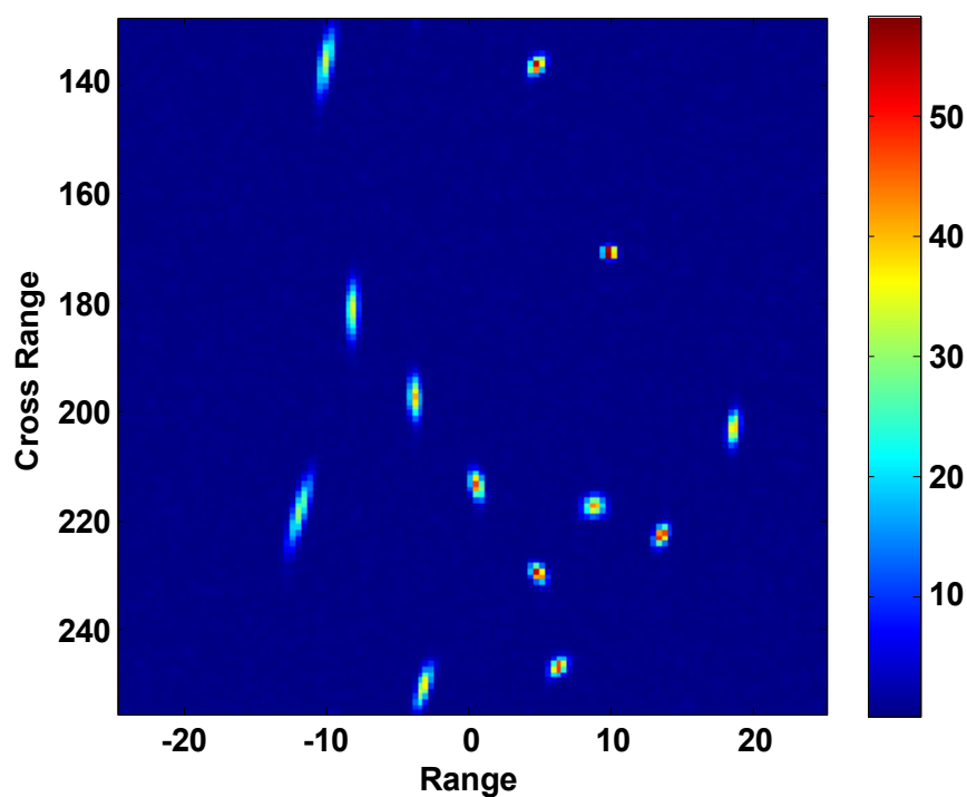
Fig.7. ISAR image using Gabor transform for F=8GHz
