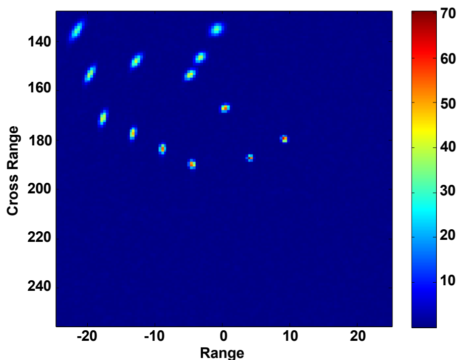
Fig.4. ISAR image using Gabor transform for F=3GHz
