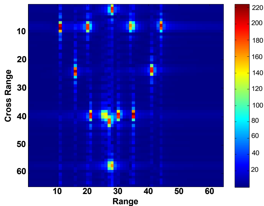
Fig.9. ISAR image using STFT for F=15GHz
