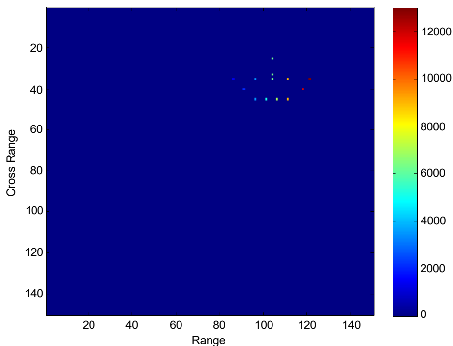
Fig.5. ISAR image using MFCFT for F=3\text{GHz}
