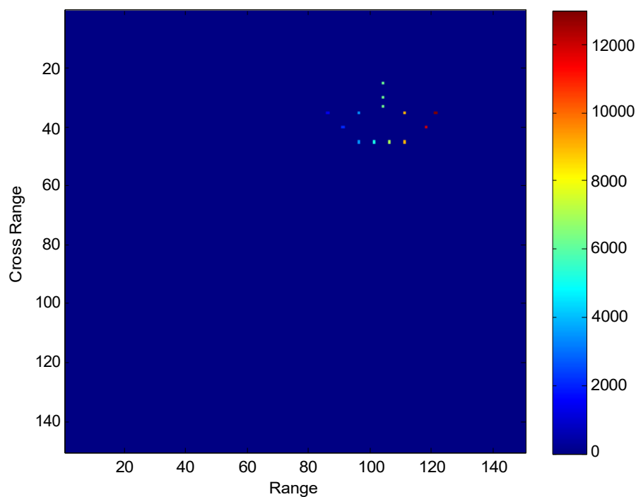
Fig.8. ISAR image using MFCFT for F=8GHz
