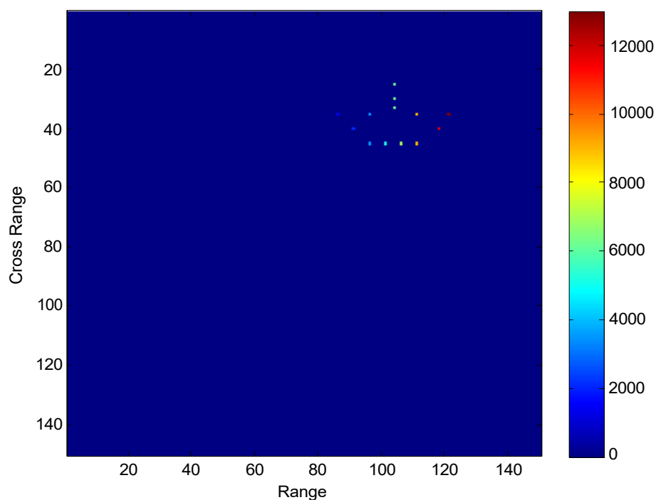
Fig.14. ISAR image using MFCFT for F=40GHz
