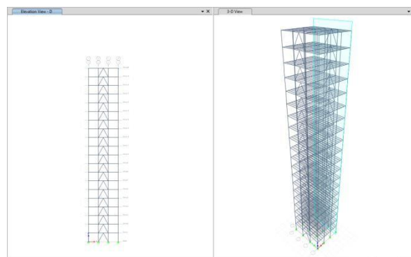
Figure 3.2 Elevation and 3D view of the building with inverted V bracings at centre bay.
