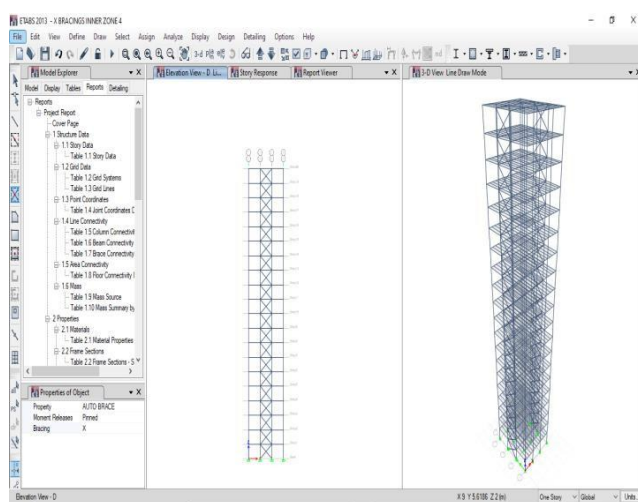
Figure 3.6 Elevation and 3D view of the building with X bracings at centre bay
