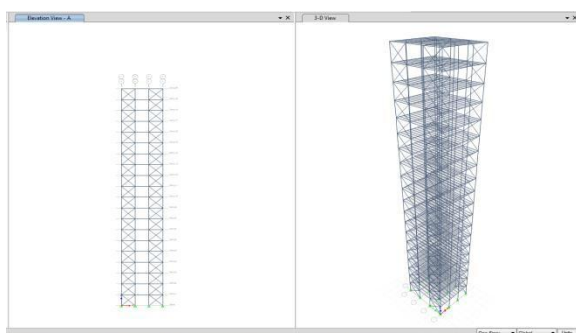
Figure 3.6 Elevation and 3D view of the building with X bracings at centre bay
