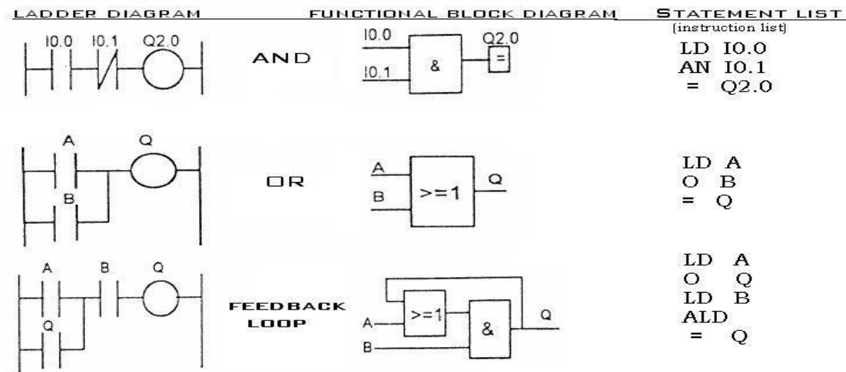
Fig 4 Example of Ladder Logic
