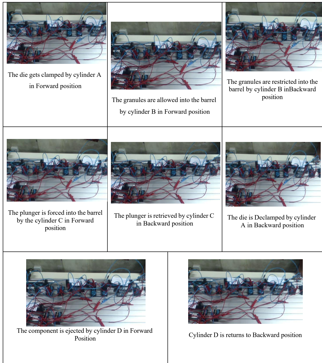
Fig 6 Automation of Injection Moulding Machine using PLC
