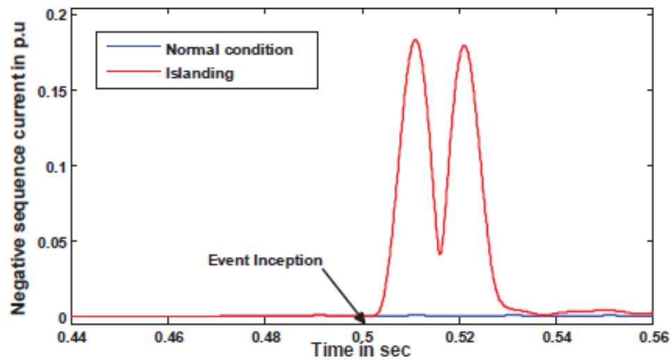
Fig.10. NSC during grid connected and islanding modes
