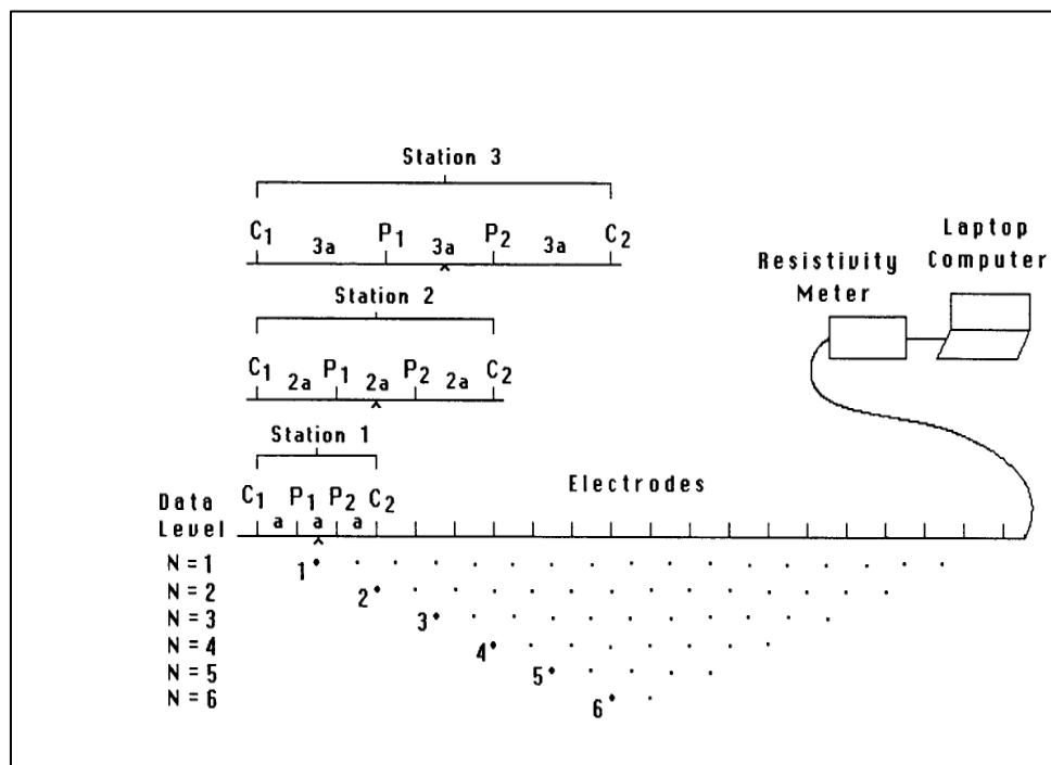
Figure 4. Measurement sequence for building a resistivity pseudo section. With an electrode spacing 'a', the first sequence of measurements are made. When this is completed, the next sequence of measurements employs the electrode spacing of '2a'. This procedure is repetitive, with increasing electrode spacing employed for each sequence. As electrode spacing increases, depth of subsurface imaged increases. Apparent resistivity values are plotted on the pseudosection with N, a multiple of the unit electrode spacing, serving as a measure of depth (Loke and Barker, 1995)
