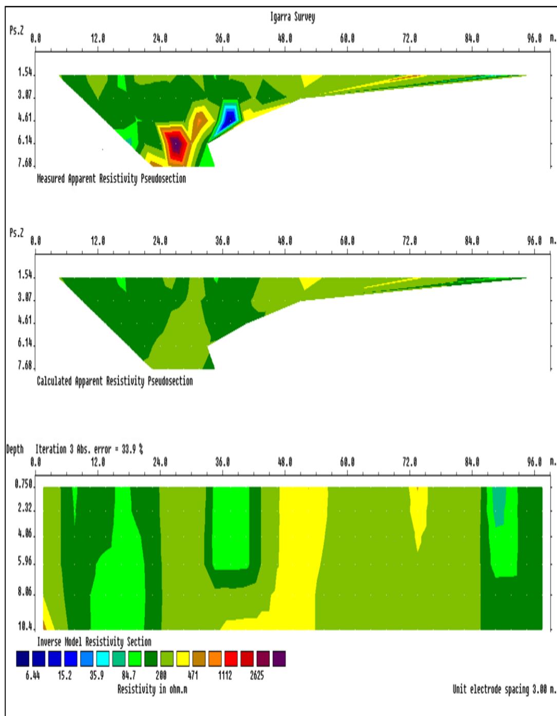
Figure 5. Measured apparent resistivity pseudosection (A), calculated apparent resistivity pseudosection (B) and inverse model resistivity section (c) for Igarra survey line (depth in meters)
