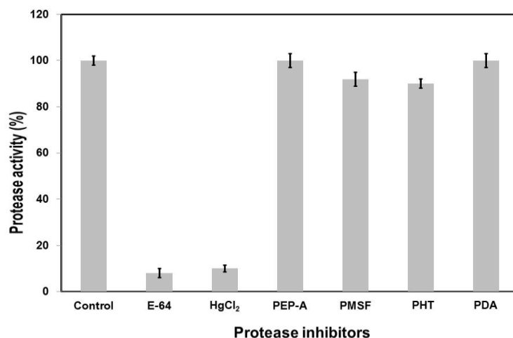
Figure 7. Effect of different protease inhibitors on the activity of the purified protease (3.2 \mu g in test). The inhibitory effect was determined by pre-incubating each of the inhibitors with the enzyme. The residual protease activity was determined by the otherwise standard Protease Assay . The corresponding activity obtained in the absence of inhibitor was taken as the control with 100% activity. Inhibitors and their concentrations tested were: E-64, 300 \mu M; HgCl 2 , 2.5 mM; PEP-A (Pepstatin A), 10 \mu M; PMSF (Phenyl methyl sulphonyl fluoride), 10 mM; PHT (1,10 - Phenanthroline), 10 mM and PDA (Pyridine 2,6-dicarboxylic acid), 10 mM.
