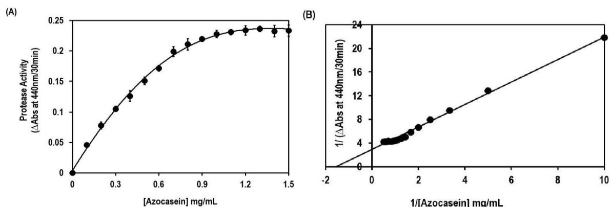
Figure 3: Substrate saturation kinetics behaviour of the purified protease using azocasein as the substrate (A) Hyperbolic substrate saturation curve of the protease (0.89 \mu\text{g/mL} protein in test). (B) The corresponding double reciprocal plot of the data of Figure 3(A) .
