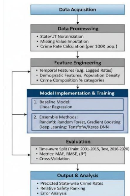
Fig. 1 Flowchart for Safe State Crime Prediction IV.
